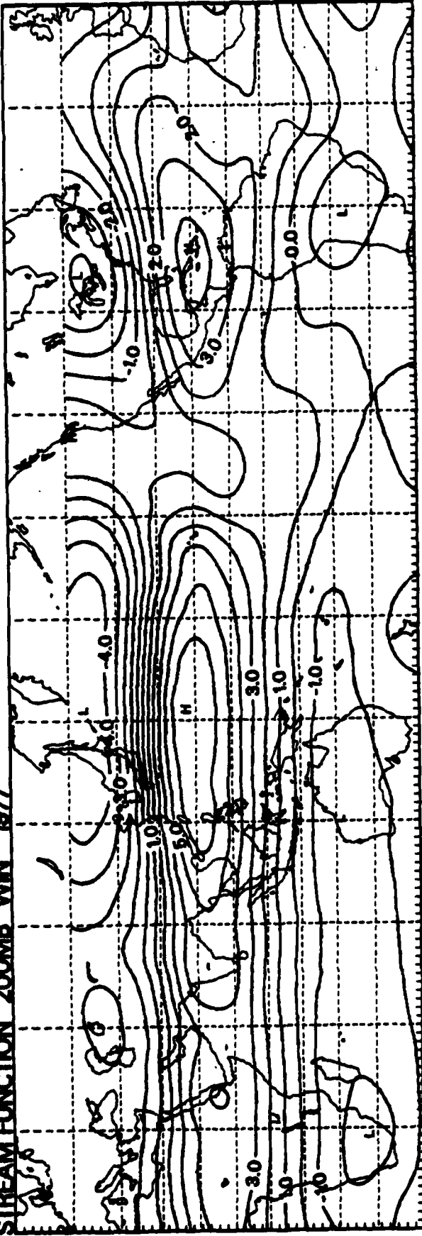
STREAM FUNCTION 200MB WIN 1977
